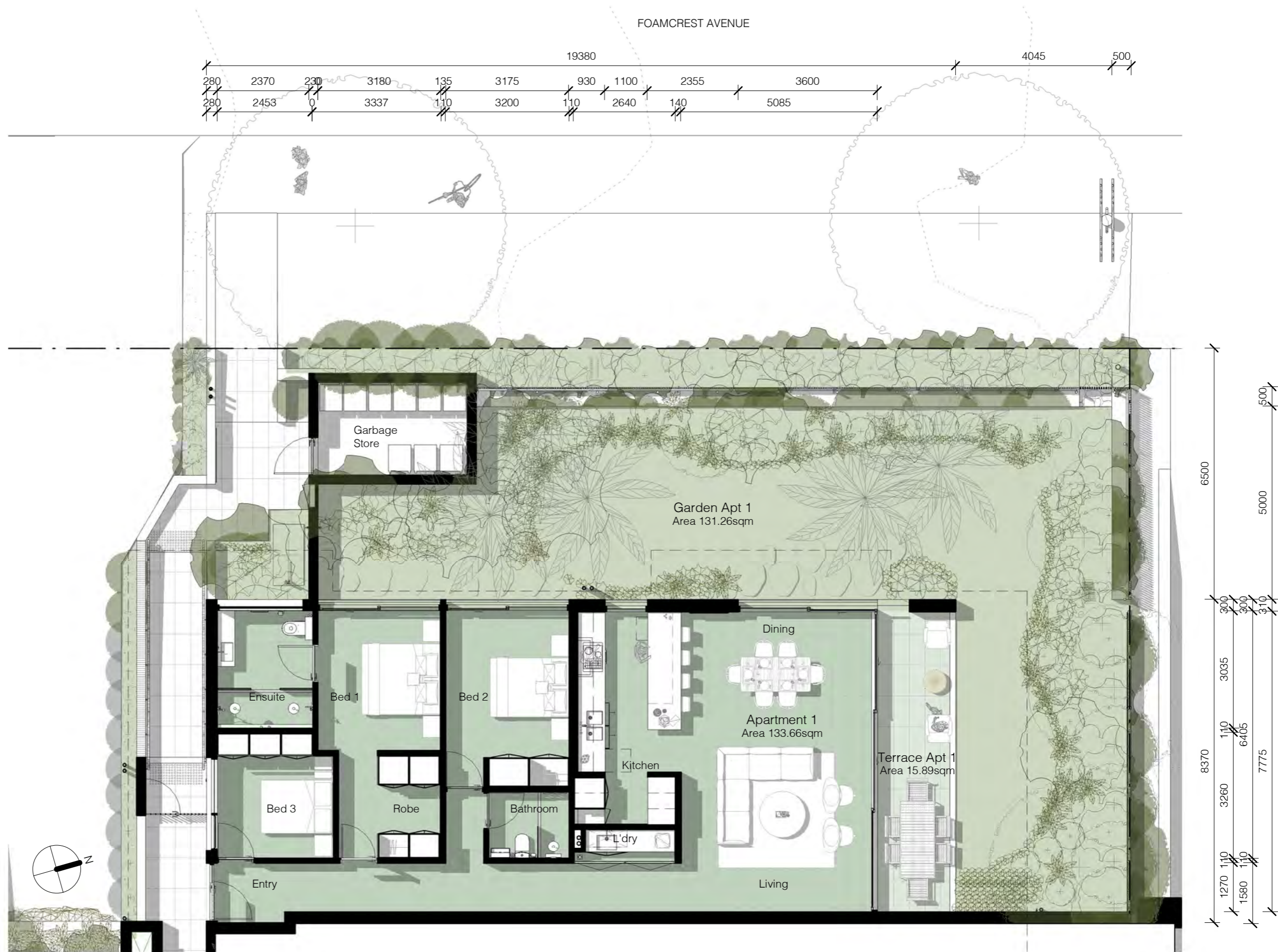
1 Apartment 1 Plan 1:100
