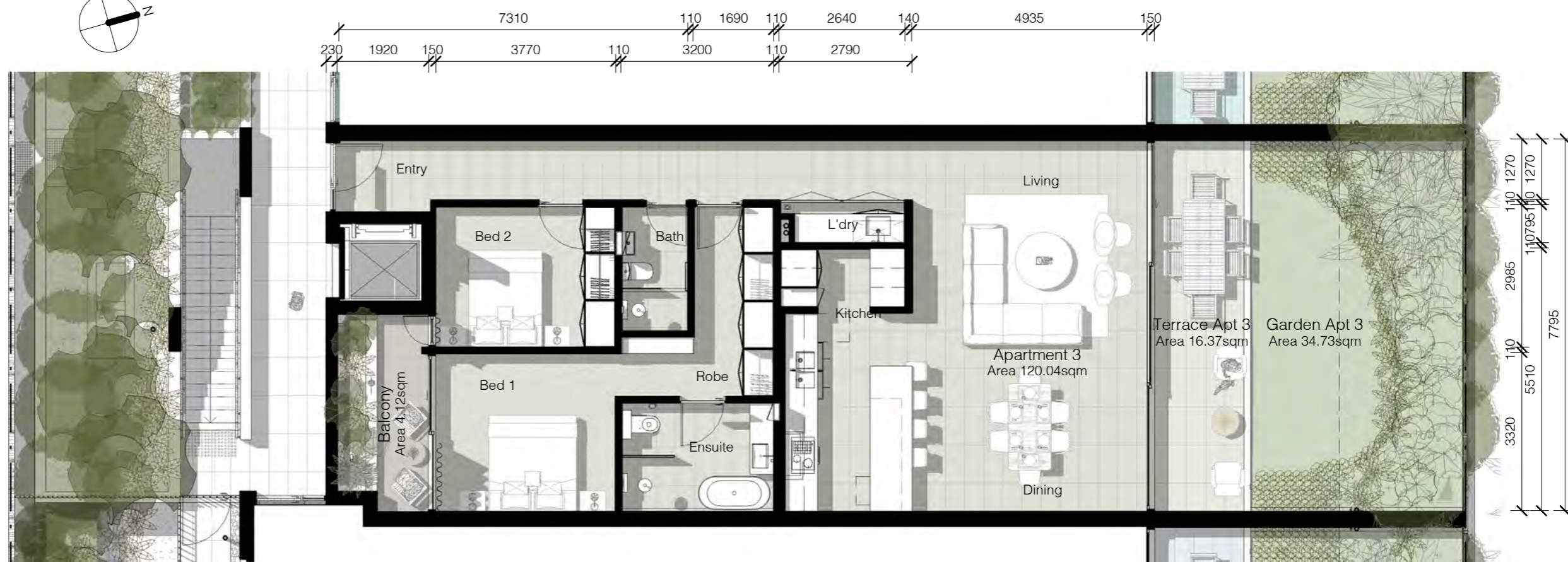
1 Apartment 3 Plan 1:100
